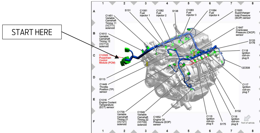
Figure 2 – Front View of Engine.
